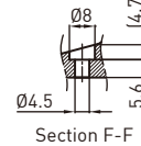
Section F-F
